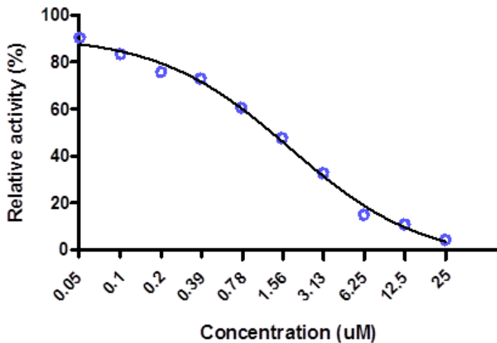
Figure 2. Inhibition of Papain-like protease activity by GRL0617 as measured with SensoLyte® 520 SARS-CoV-2 Papain-like Protease/Deubiquitinase Activity Assay Kit.
